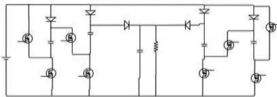
Fig.2 Topologies with Switched Capacitor (SC)
